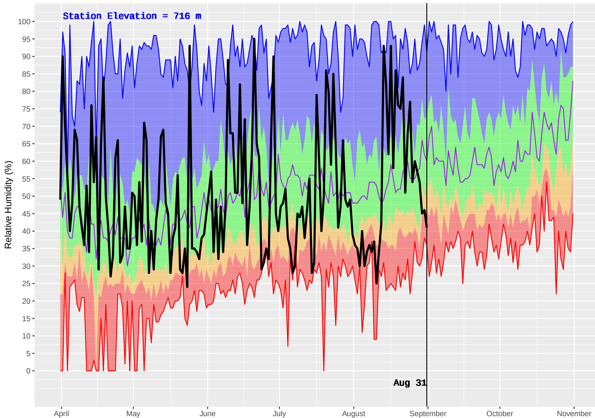
MCBRIDE HUB (195) : Historical (1980–2016) and Current (2017) Noon Relative Humidity
